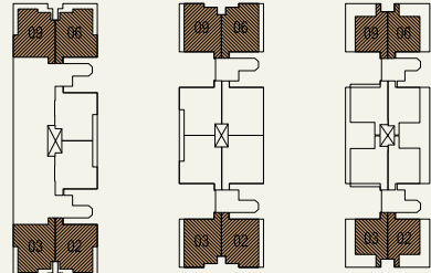
4TH STOREY PLAN 5TH STOREY PLAN ATTIC PLAN
