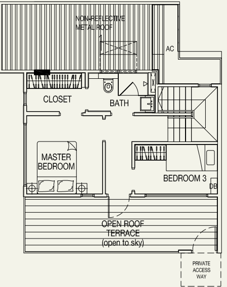
DUPLEX SECOND FLOOR
