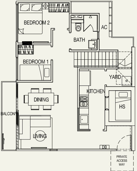
DUPLEX FIRST FLOOR
